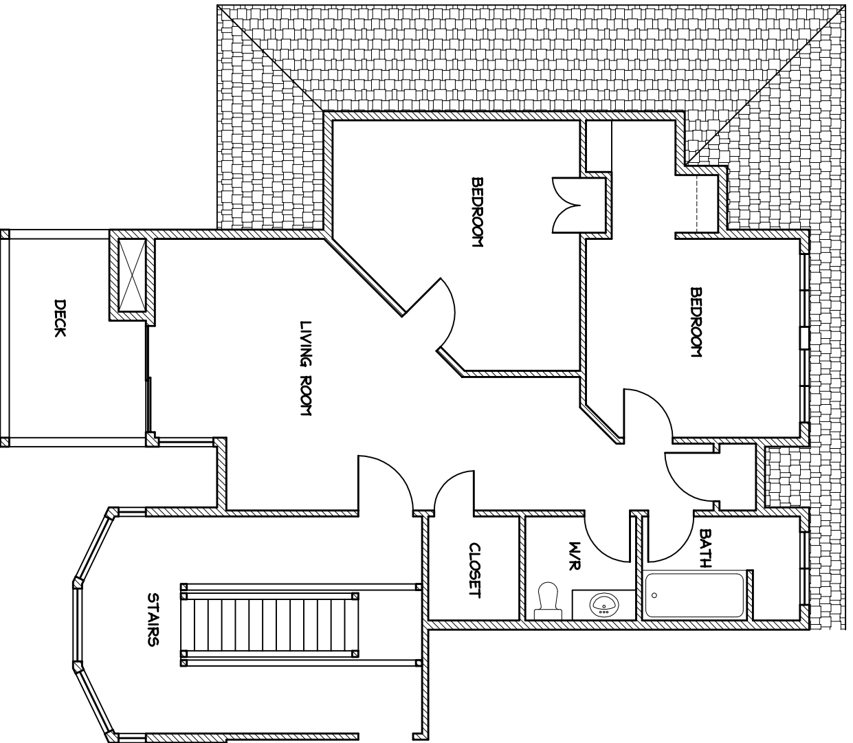
GREAT HORNED OWL 2 BEDROOM UPPER UNIT 829 SQ.FT.
