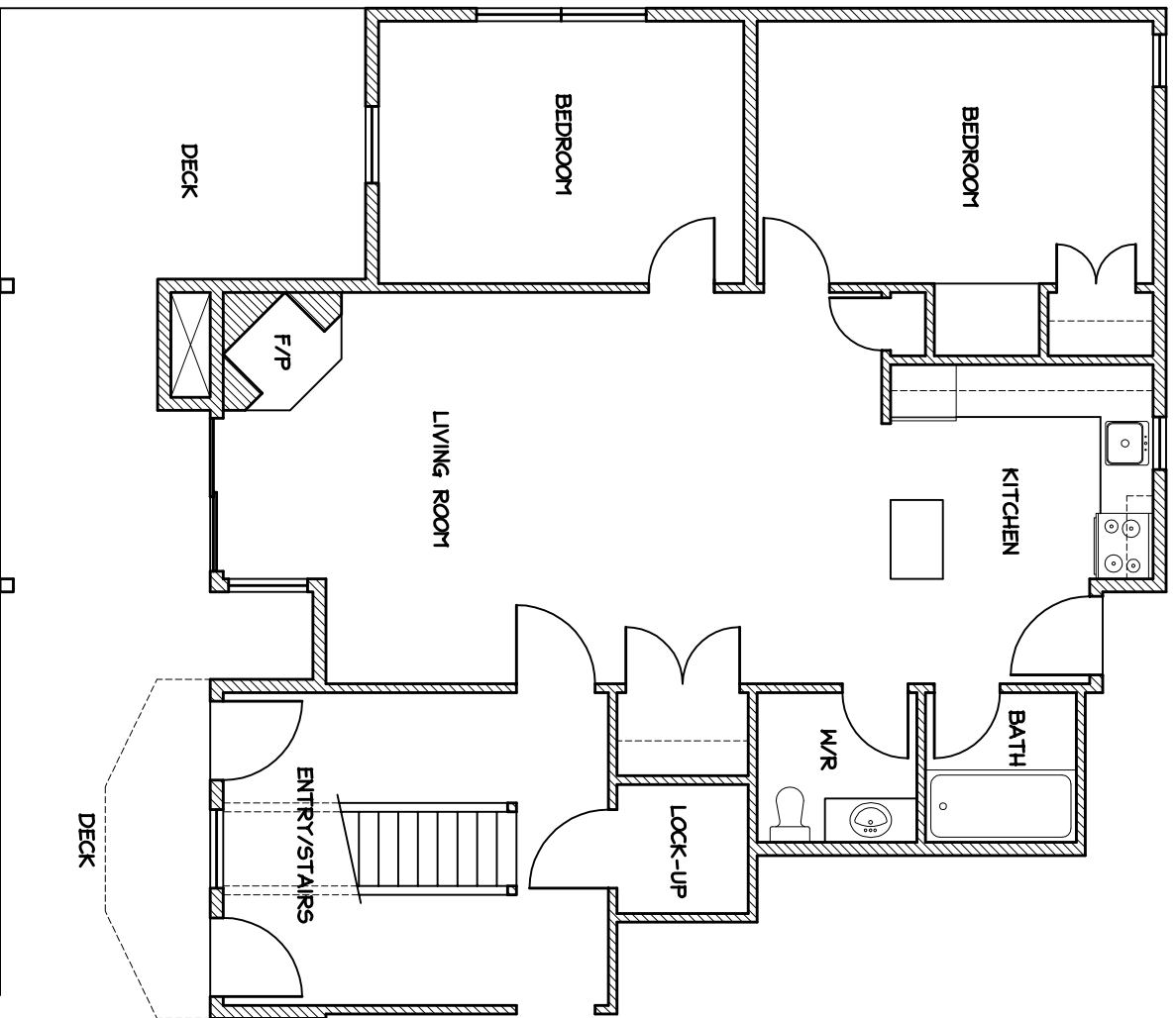
GREAT HORNED OWL 2 BEDROOM LOWER UNIT 972 SQ.FT.
