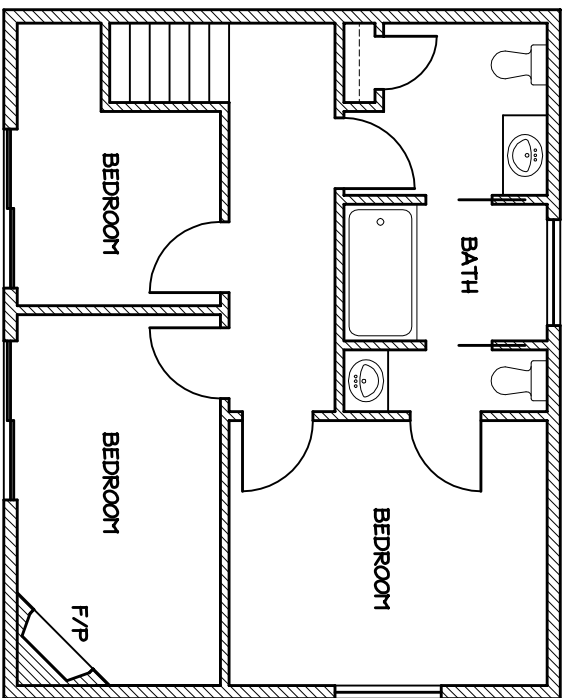
CROMS NEST COTTAGE LOWER FLOOR
